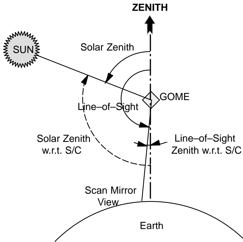
Figure 3: Zenith Angles
